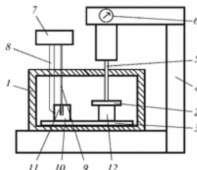
Fig. 2. Diagram of setup for performing thermomechanical tests on materials.
