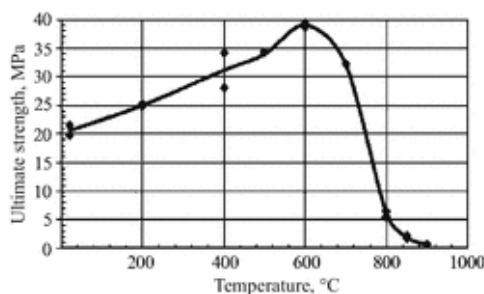
Fig. 1. Ultimate strength of a fireclay refractory (ShB-5) in compression versus temperature.
